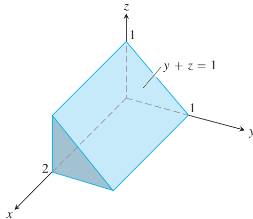
Figure 1: Prism.
